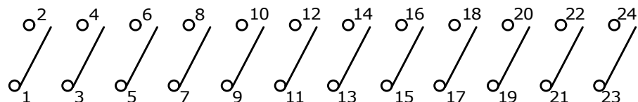
CIRCUIT - 12 POSITION
