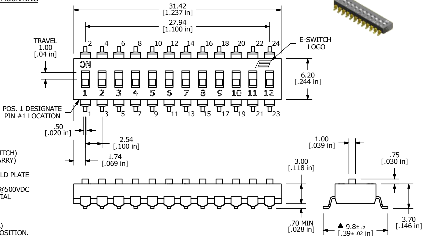
P.C.B. MOUNTING
