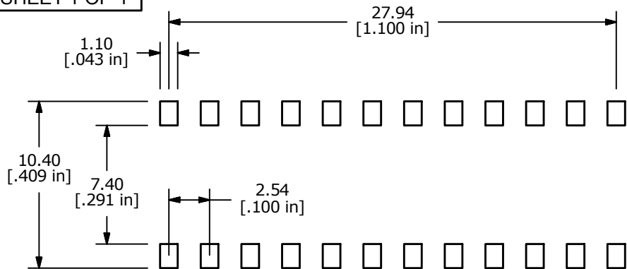
P.C.B. MOUNTING
